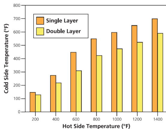
Thermal Protection - Hot Side vs. Cold Side
